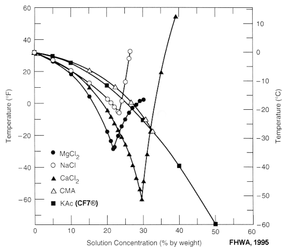
Refreeze Temperatures
